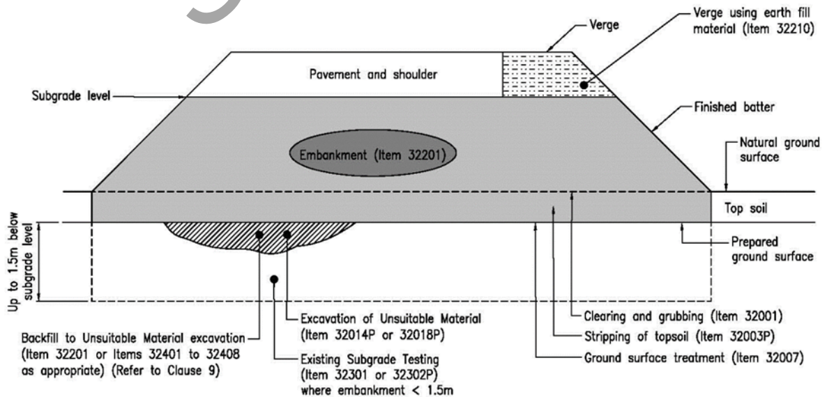
Figure 2.1(b) – Embankment
