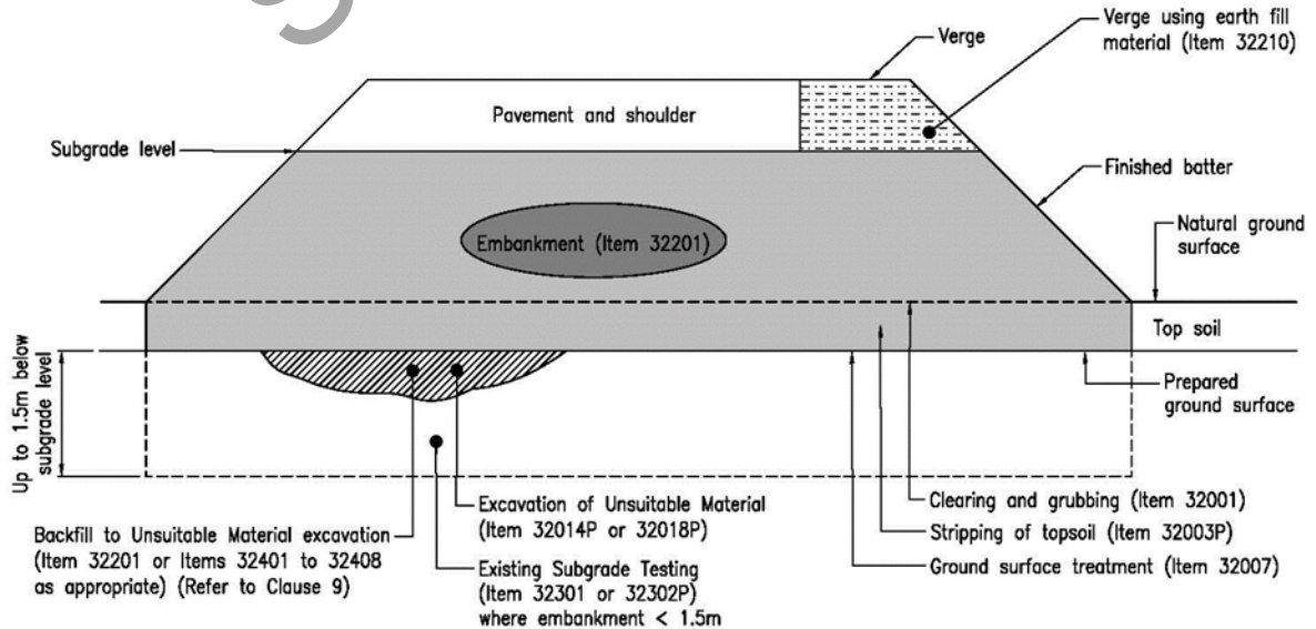
Figure 2.1(b) – Embankment
