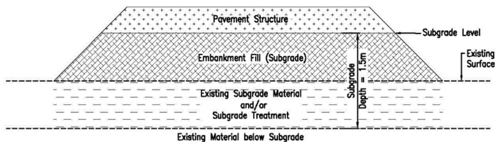
Figure 2(e) – Subgrade Depth in an embankment <1.5 m high
