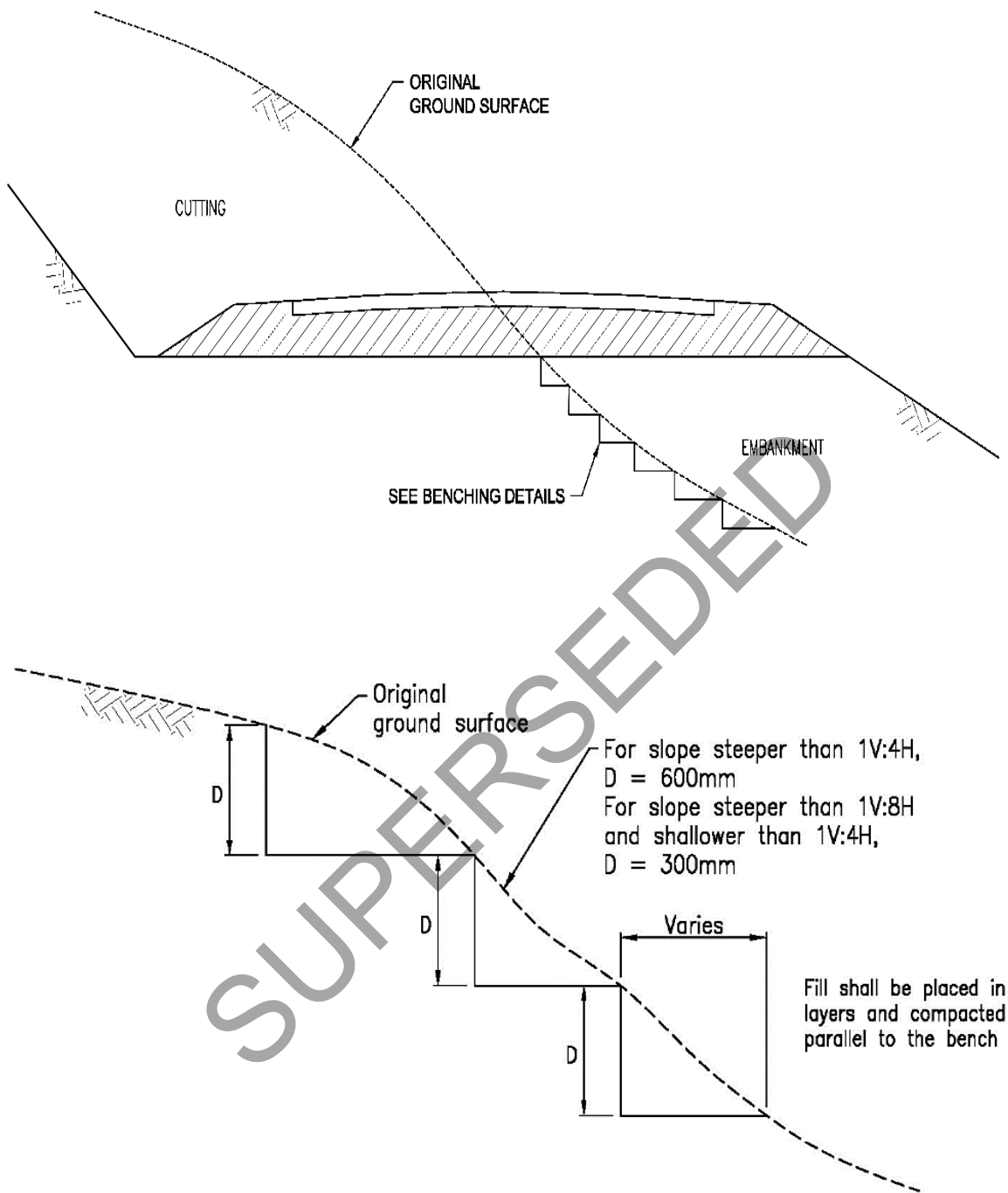
Figure 14.3.3.1 – Transverse transition in earth cutting (also applies to longitudinal transition)
