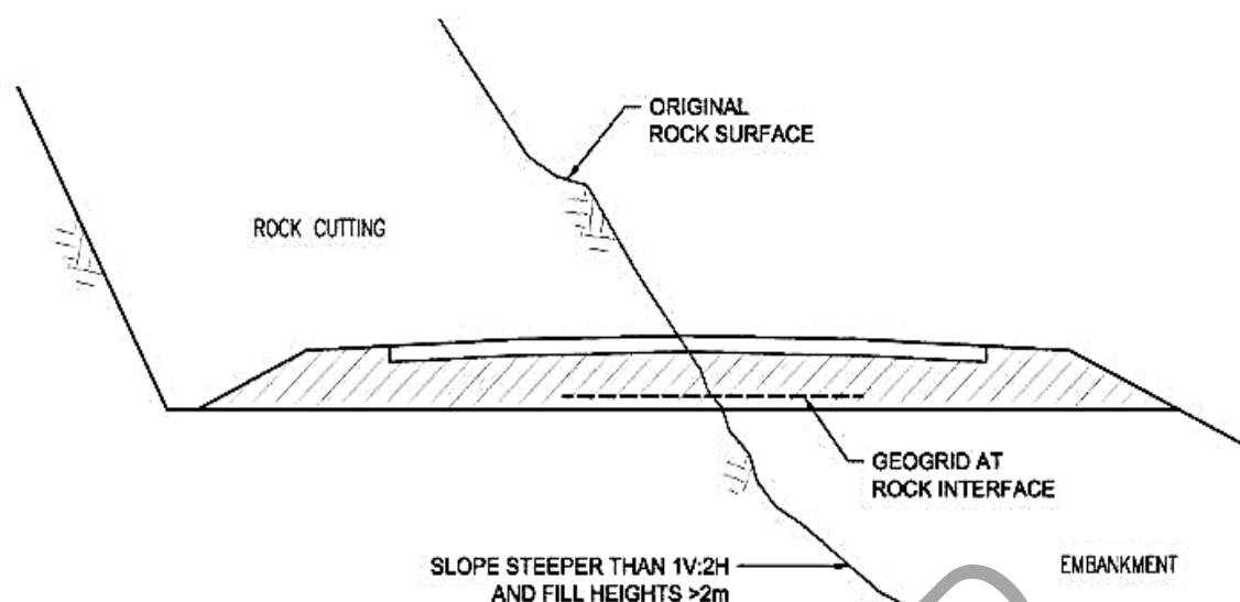
Figure 14.3.3.2 – Transverse transition in hard rock (also applies to longitudinal transition)
