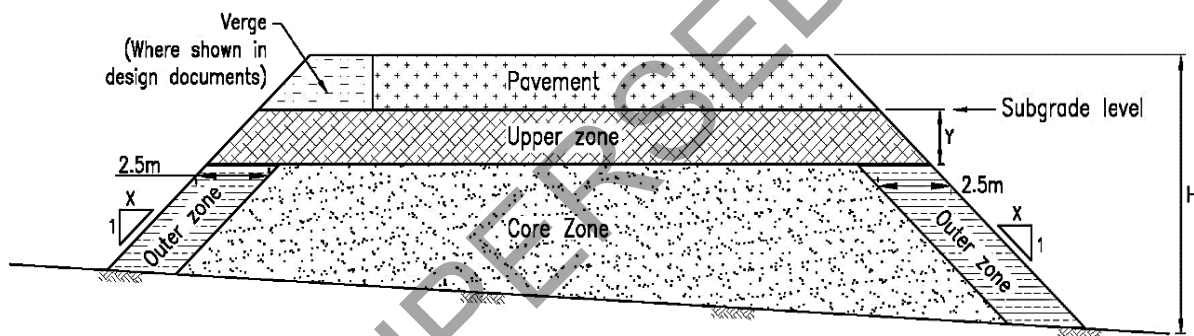
Figure 14.3.1 – Embankment zones
