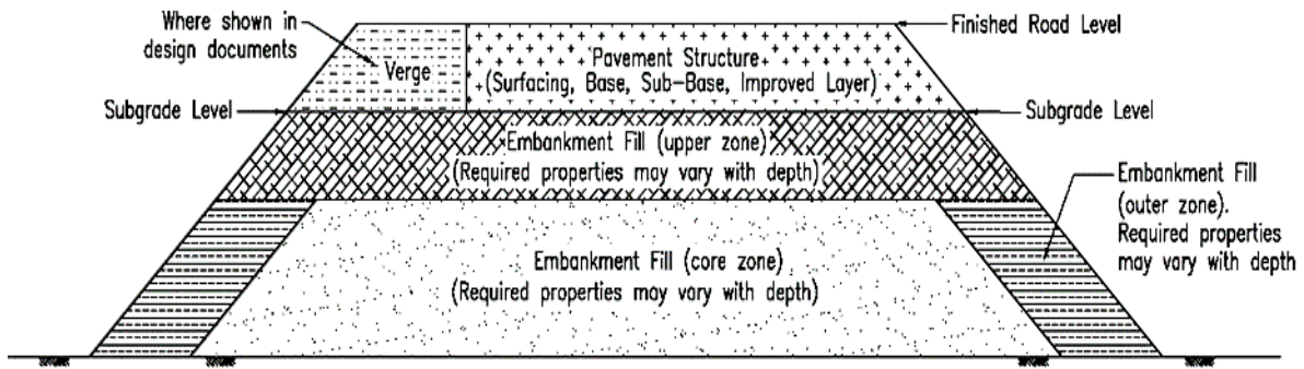
Figure 2(a) – Embankment terminology – zoned
