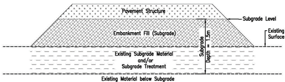
Figure 2(d) – Subgrade Depth in an embankment >1.5 m high
