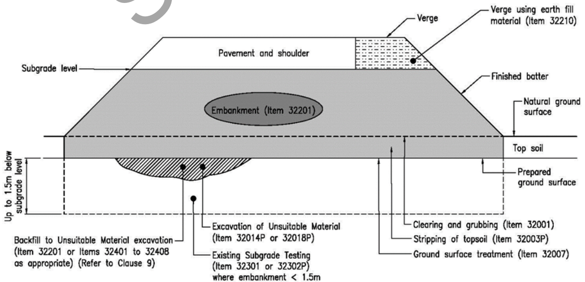
Figure 2.1(b) – Embankment
