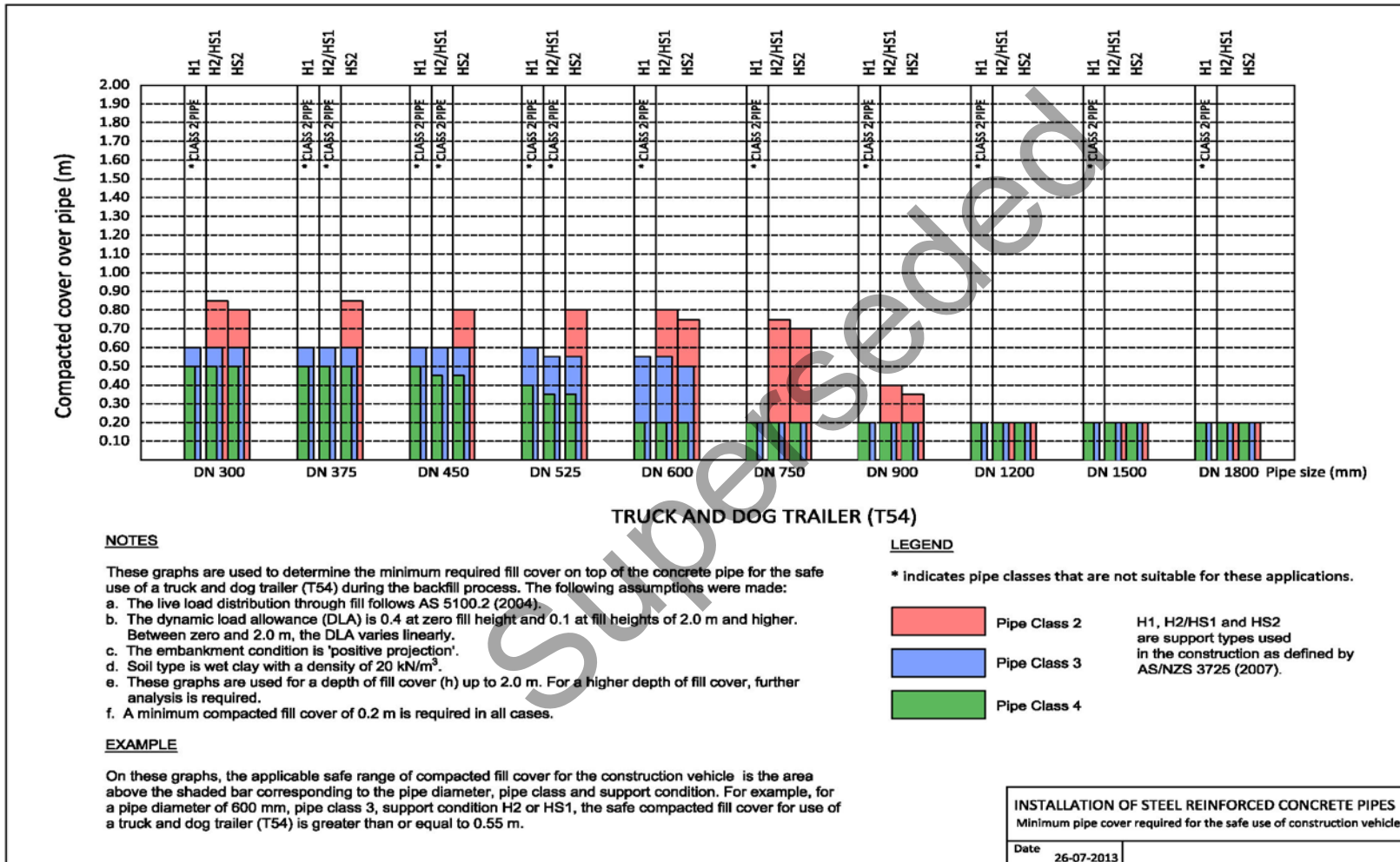
Figure B1 - Fill height and Pipe Load Class for various installation conditions for Truck and Dog Trailer
