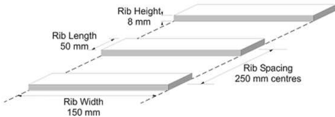
Figure 7.7.3(a) – ATLM edge line
