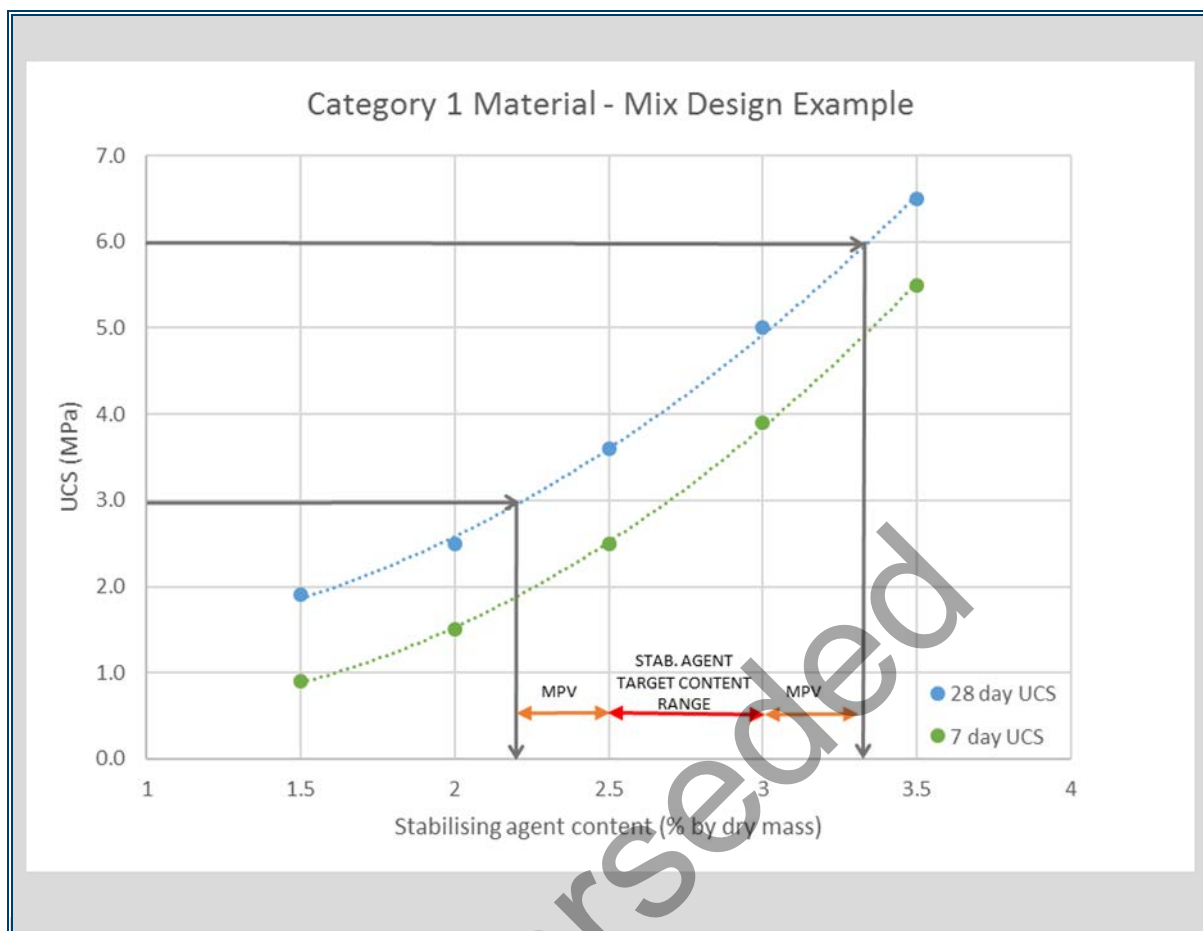
Figure 7.3.1 – Mix design example (Category 1 material)
