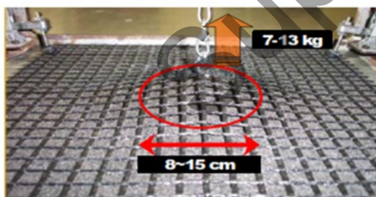
Figure 10.2.5 – Spring balance test to measure the construction bond strength
