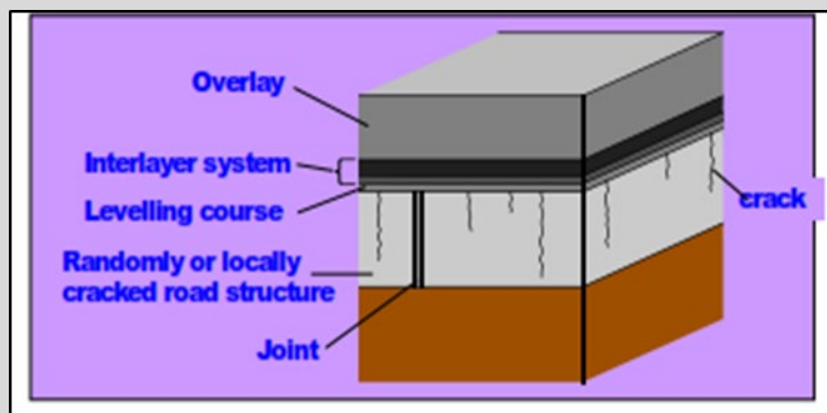
Figure 1(d) – Schematic of reflective cracking treatment
