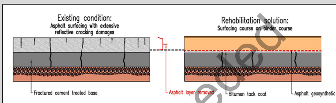
Figure 1(e) – Example of reflective cracking treatment
