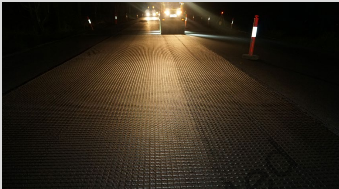
Figure 9.4.2(b) – Example of roller being used for the initial bedding of the asphalt geosynthetic
