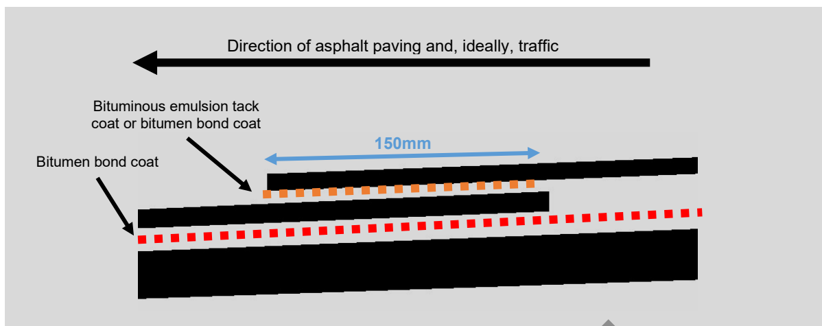
Figure 9.4.3 – Asphalt geosynthetic overlaps
