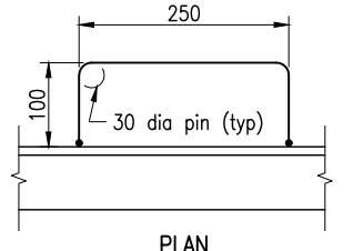
HANDLE DETAIL
