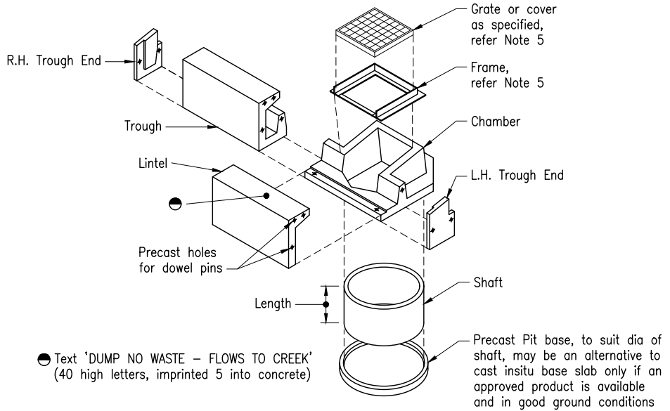
TYPICAL PRECAST COMPONENT ASSEMBLY
