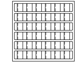
PLAN - GRATE shown in left flow situation. For right flow, rotate grate through 180°. TYPICAL VANED GRATE (Bicycle Safe)
