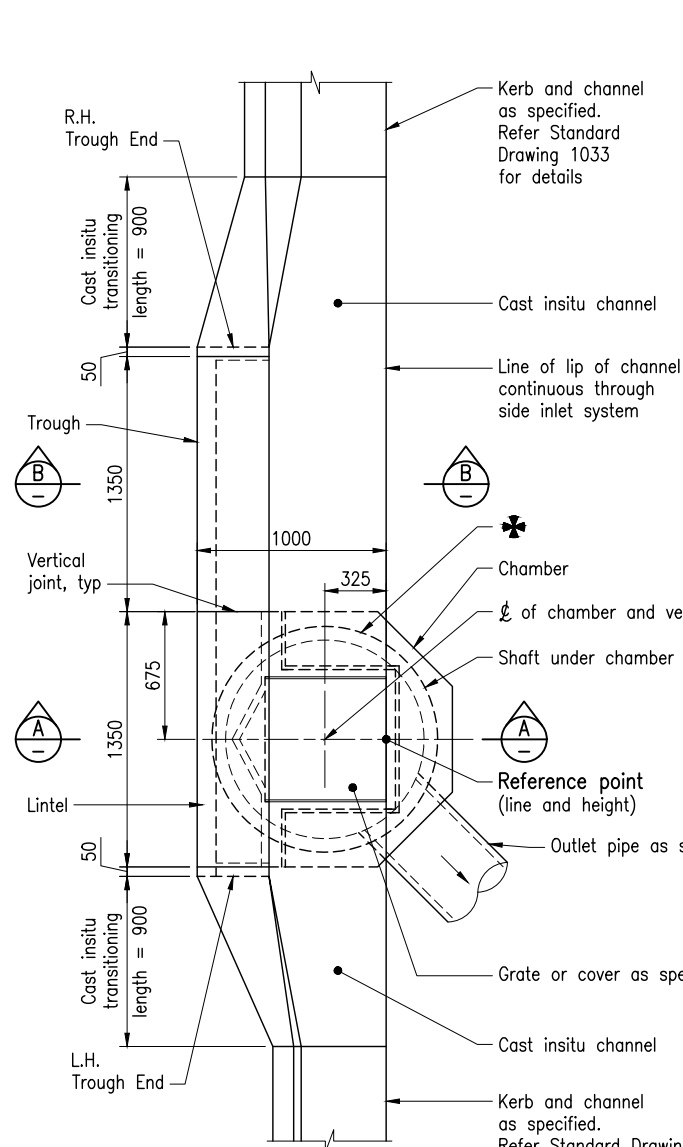
TYPICAL PLAN INSTALLED SIDE INLET GULLY
