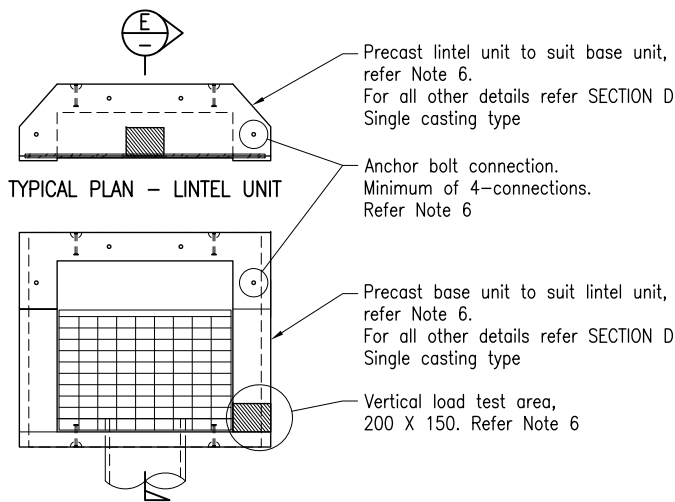
TYPICAL PLAN - BASE UNIT ALTERNATIVE DETAIL FOR SEPARATE LINTEL AND BASE UNIT
