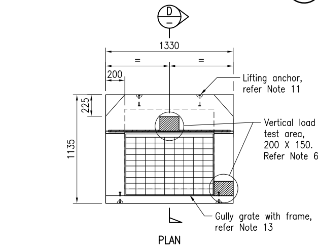
PLAN PRECAST ANTI-PONDING INLET UNIT
