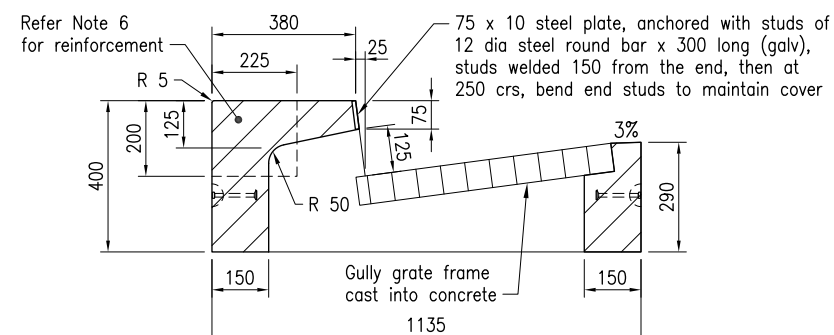
SECTION D SINGLE CASTING
