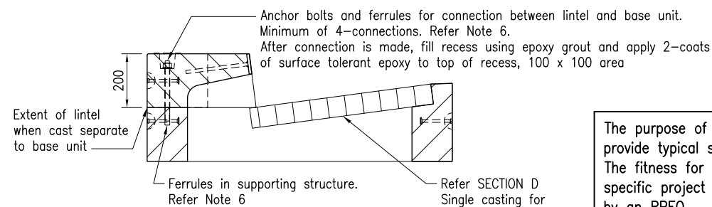
SECTION E ALTERNATIVE DETAIL FOR SEPARATE LINTEL AND BASE UNIT Refer Note 6
