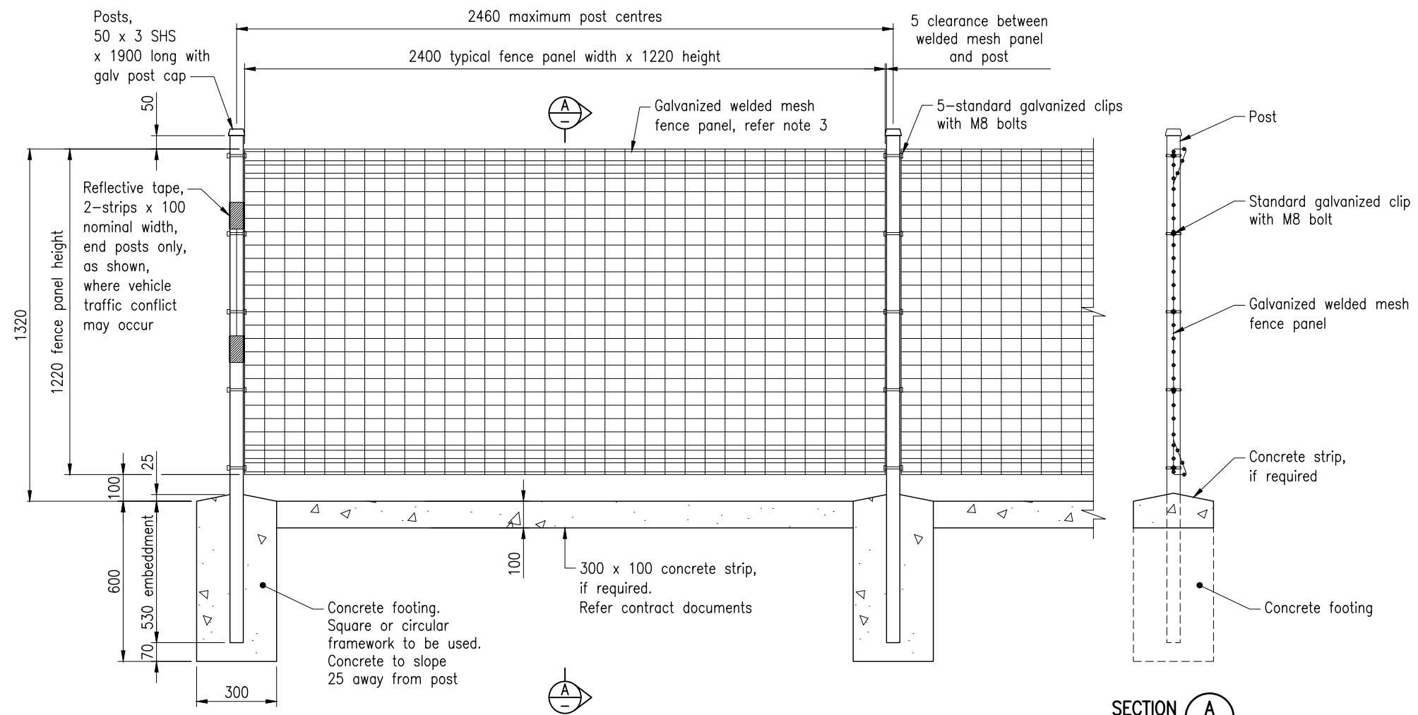
PART ELEVATION GENERAL ARRANGEMENT
