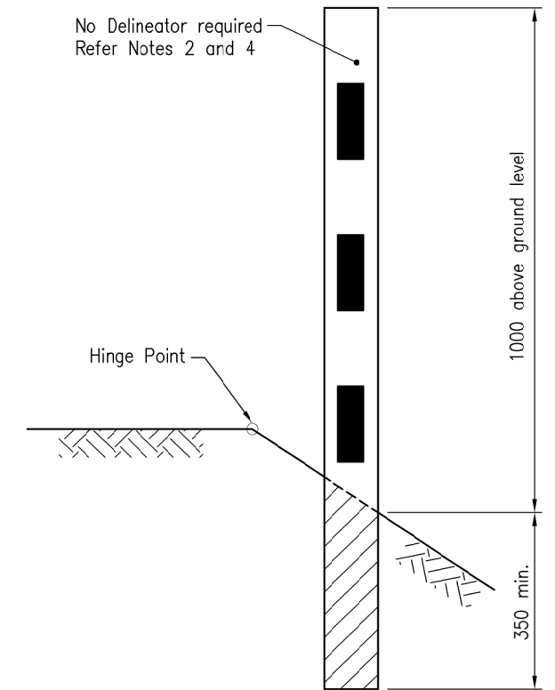
POST LOCATED BEYOND HINGE POINT
