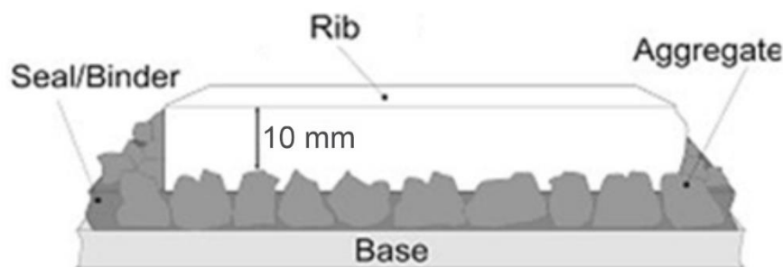
Figure 7.7.3(c) – Height measurement of the raised rib
