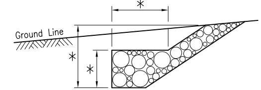
ALTERNATE TOE WALL DETAILS - TYPE B
