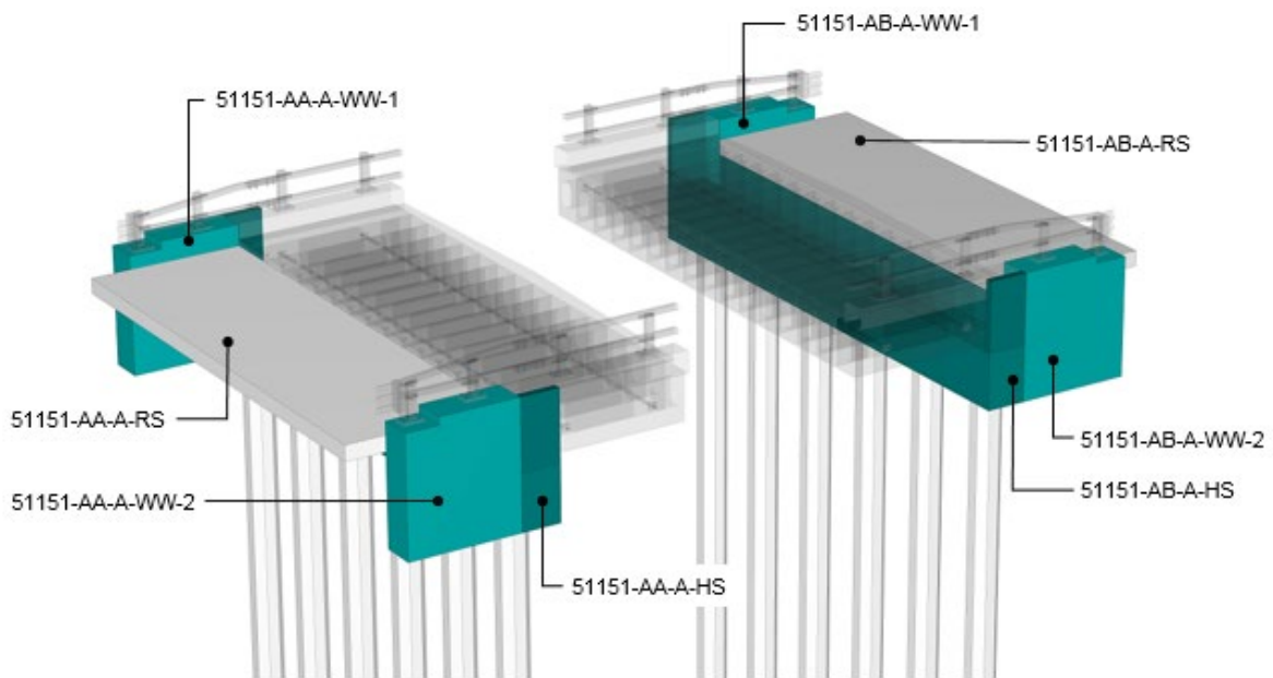
Figure 5.2.2.2(b) – Object naming convention for abutments with multiple wingwalls
