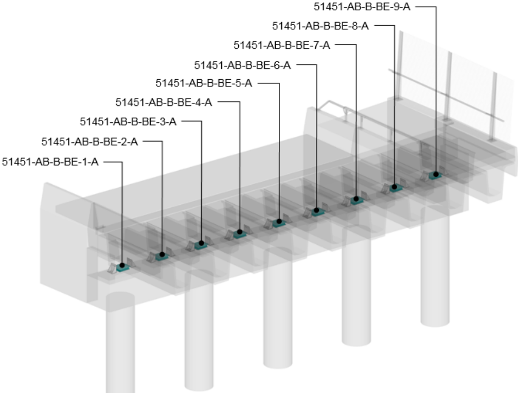
Figure 5.2.2.4(c) – Naming convention for bearing objects
