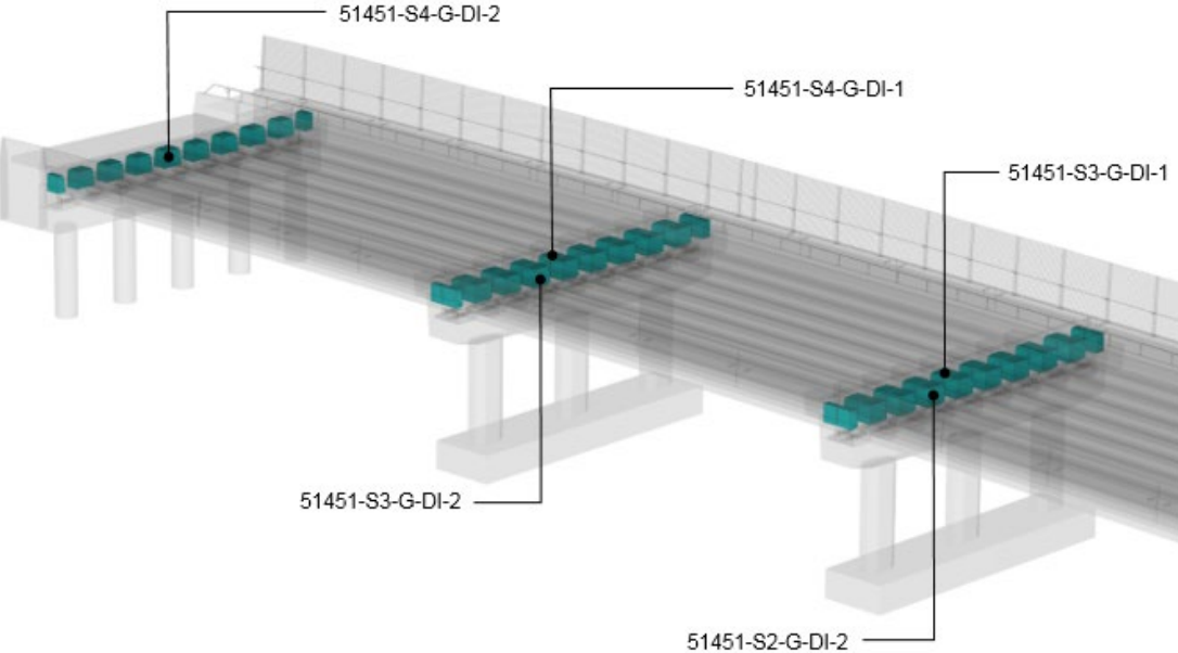
Figure 5.2.3.1(c) – Naming convention for concrete diaphragm objects
