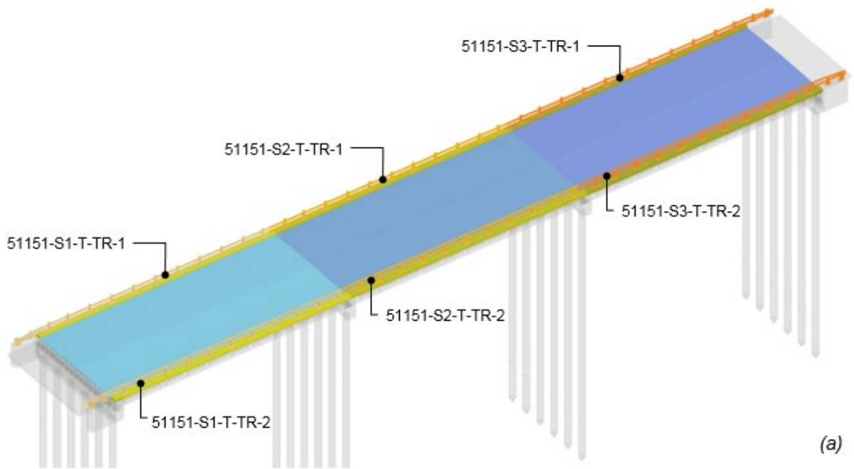
Figure 5.2.3.3 – Naming convention for bridge barrier objects
