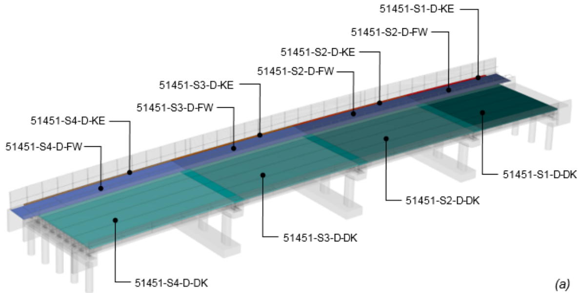
Figure 5.2.3.2(b) – Naming convention for bridge deck objects
