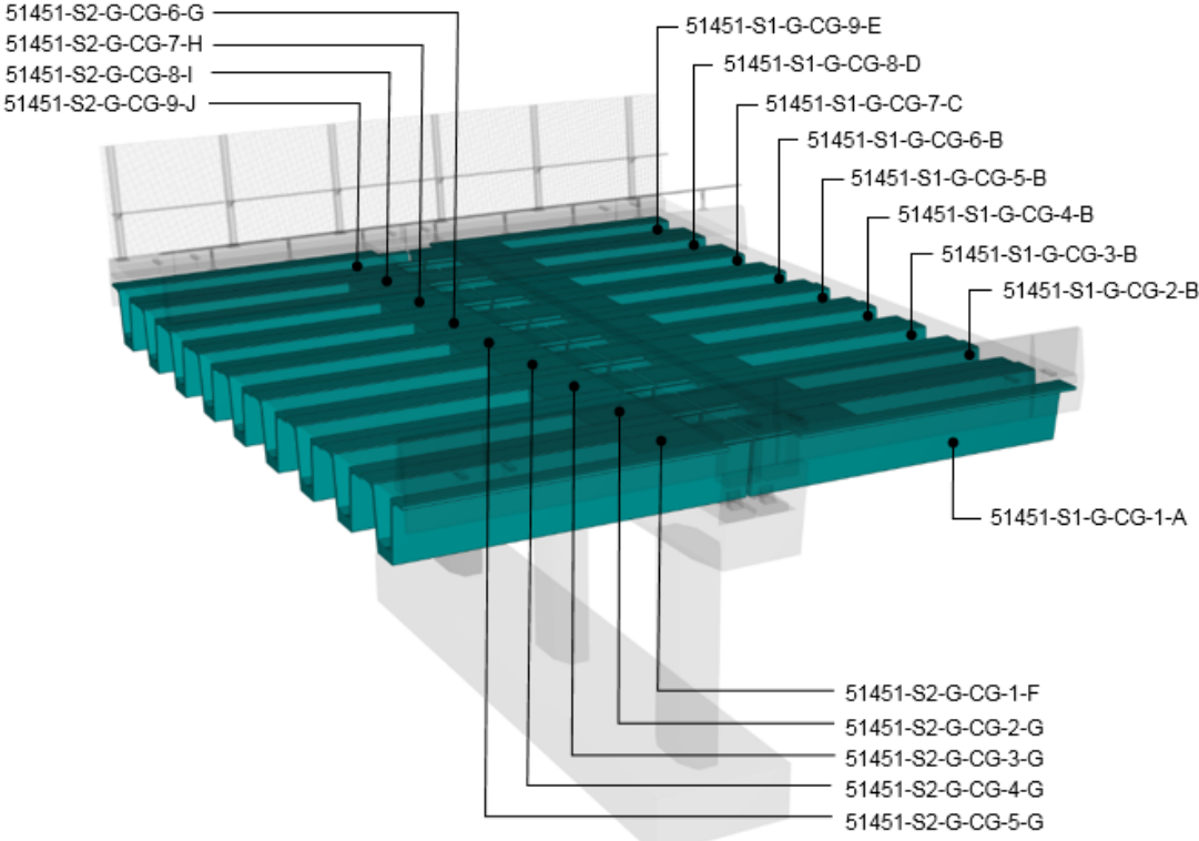
Figure 5.2.3.1(b) – Naming convention for concrete girder (Super-T) objects
