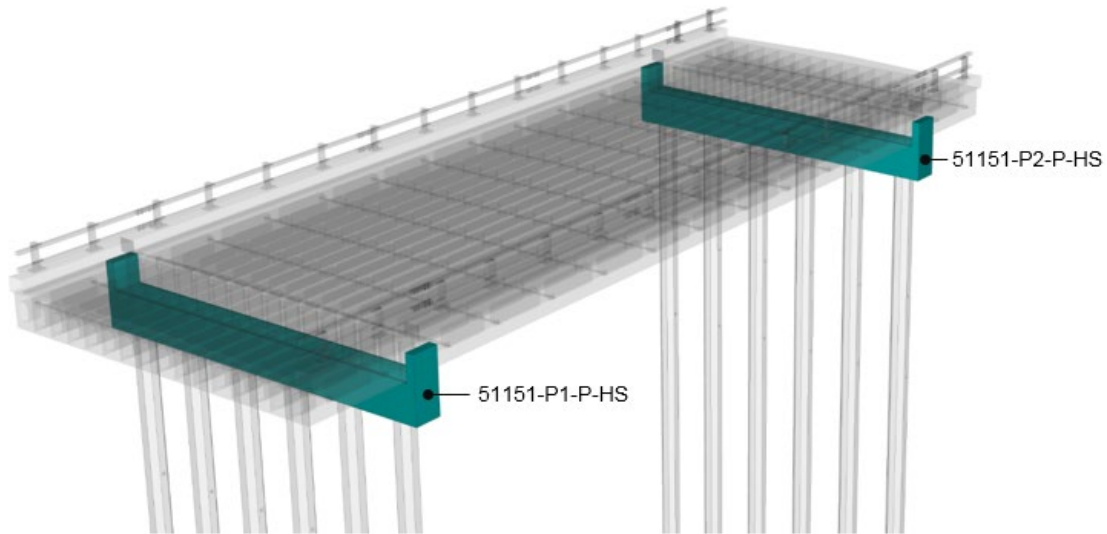
Figure 5.2.2.3(b) – Object naming convention for piers with columns
