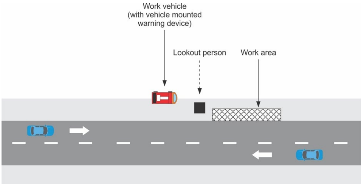
Figure 5.4.1(b) – Short-term works outside a traffic lane (works greater than 1.2 m from a traffic lane)
