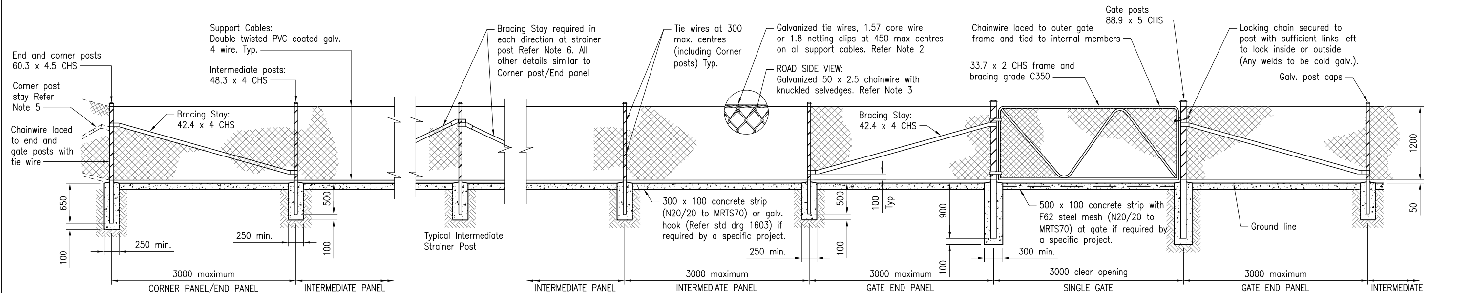
1200 HIGH FENCE
