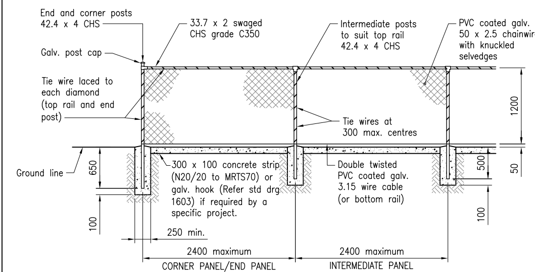
1200 HIGH FENCE WITH TOP RAIL
