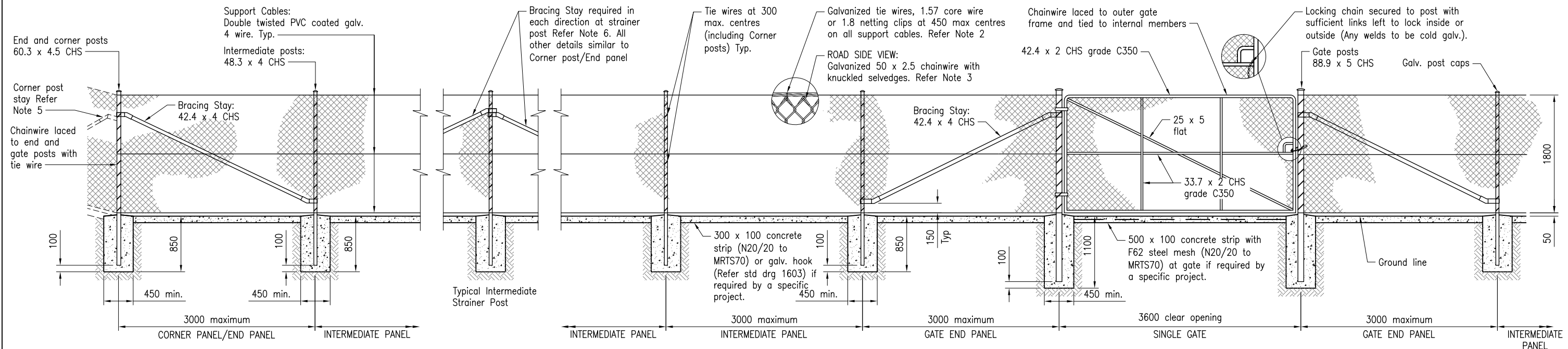
1800 HIGH FENCE
