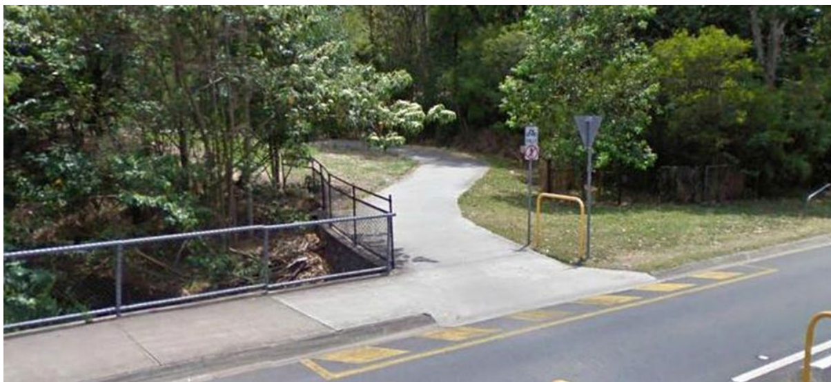
Figure C.11 – Example of terminal appearance treatment using pavement markings
